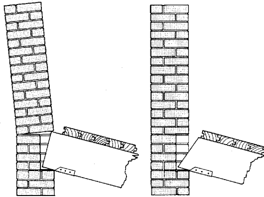
FIGURE 4.10 A timber beam that burns through in a prolonged fire is likely to topple its supporting masonry wall (left) unless its end is firecut (right). The beam is anchored to the wall in each case by a steel strap anchor of the type shown in Figure 4.13
