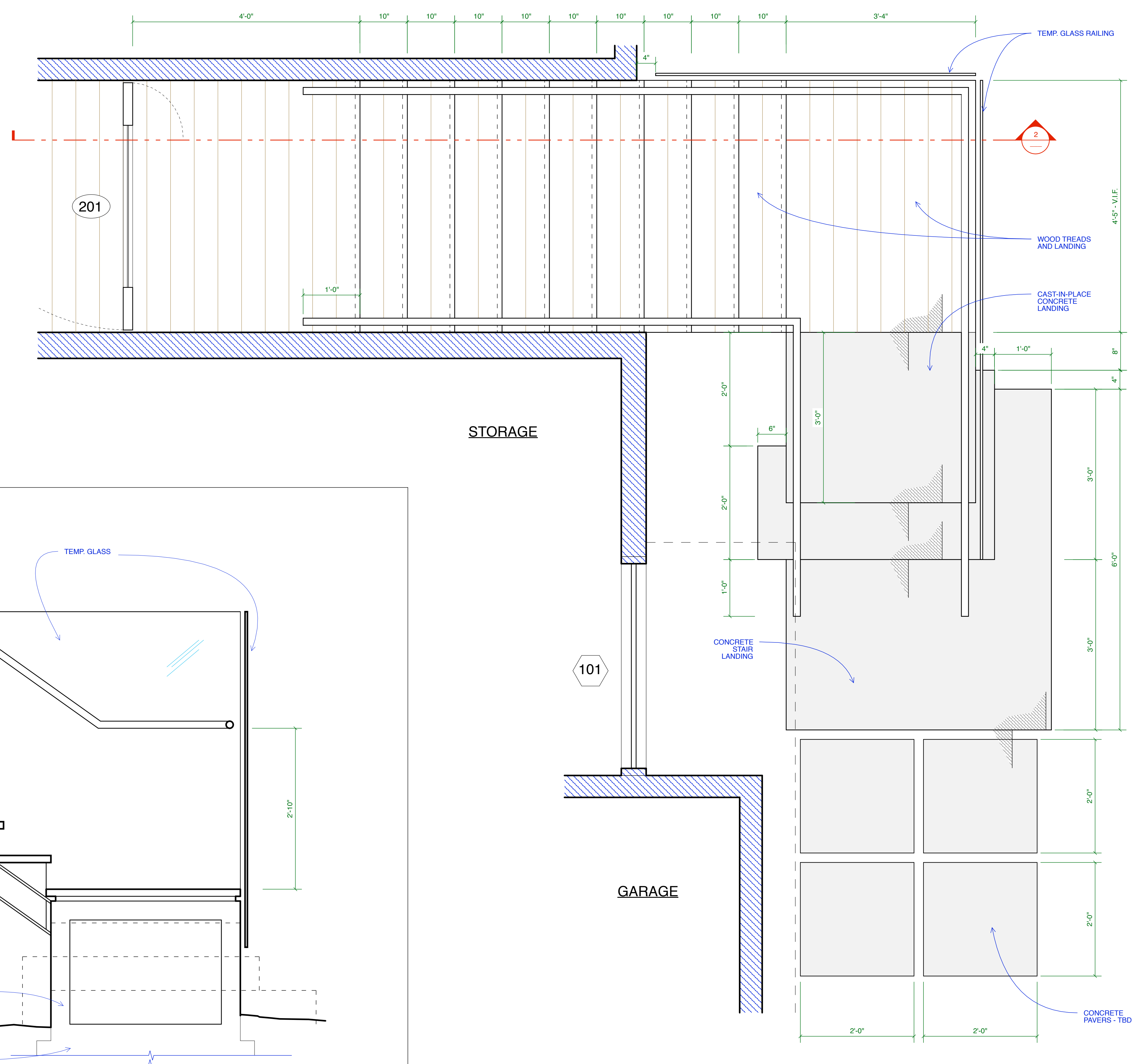
ENLARGED STAIR SECTION SCALE: 1" = 1'-0"
