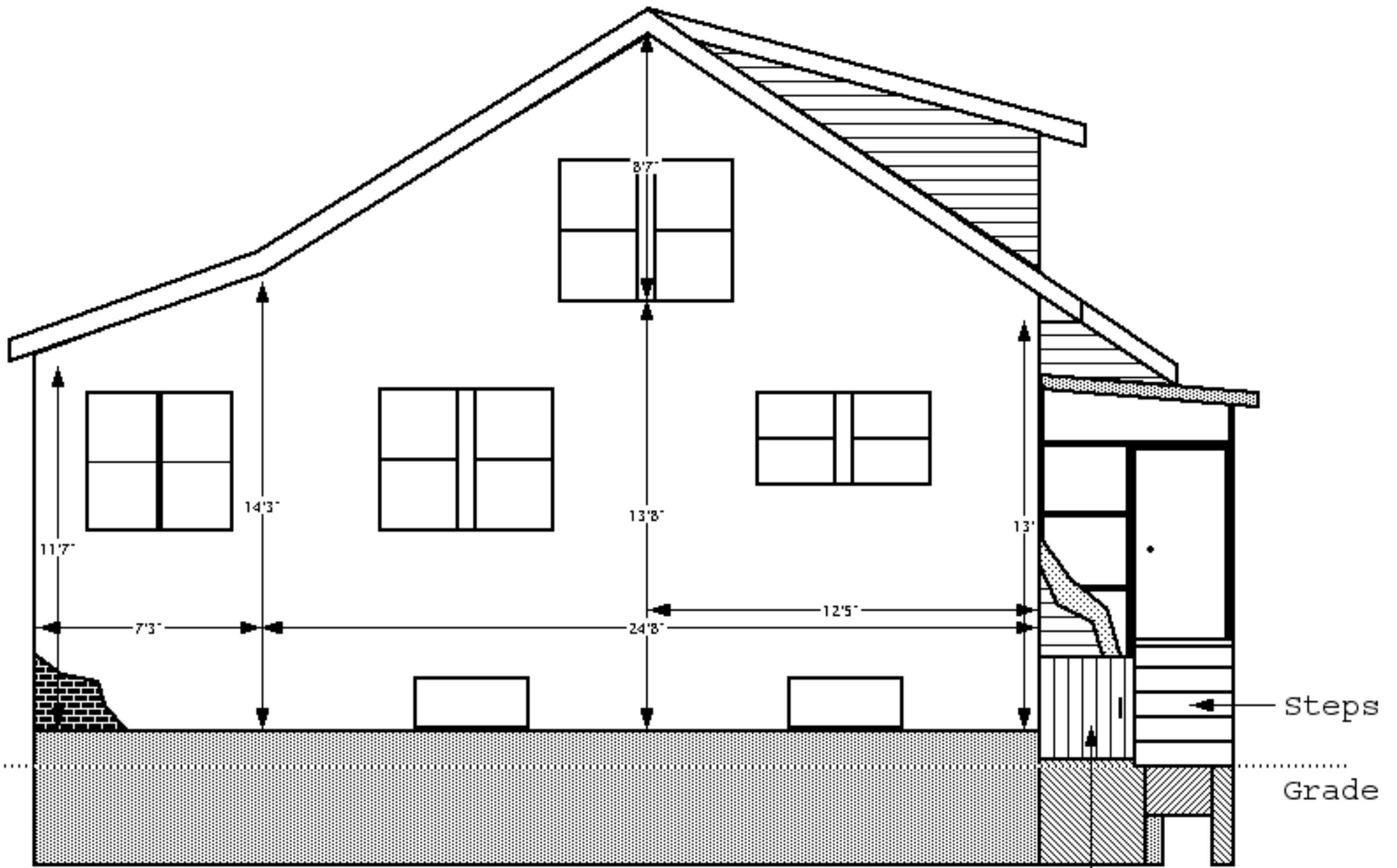
North Elevation Planned
