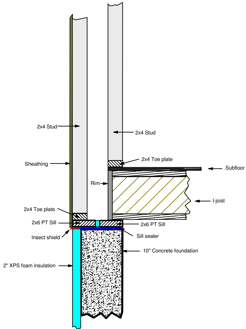
Detail at Foundation Perpendicular to Joists
