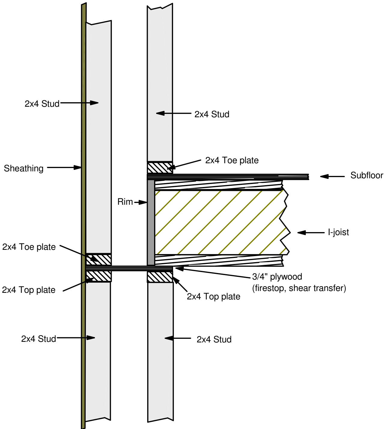
Detail of Wall Between Floors View Perpendicular to Joists
