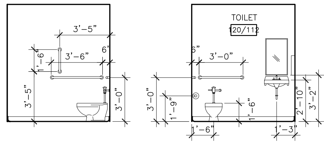
2 TOILET ROOM ELEVATIONS SCALE: 1/4" = 1'-0"
