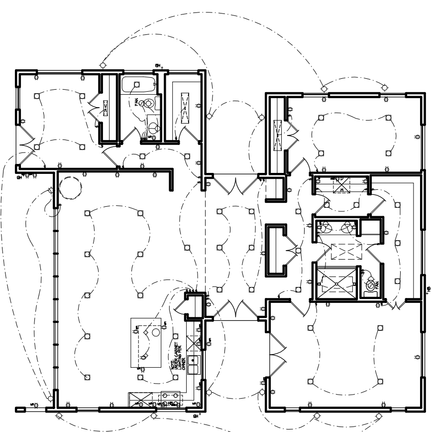
ELECTRICAL PLAN 1/4" = 1'-0"
