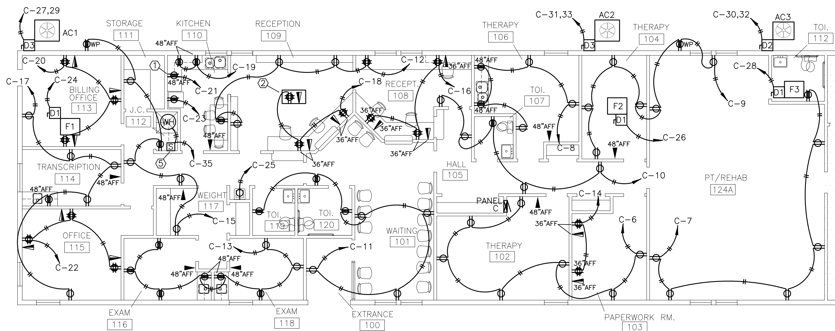
1 1ST FLOOR POWER PLAN SCALE: 1/8" = 1 FT
