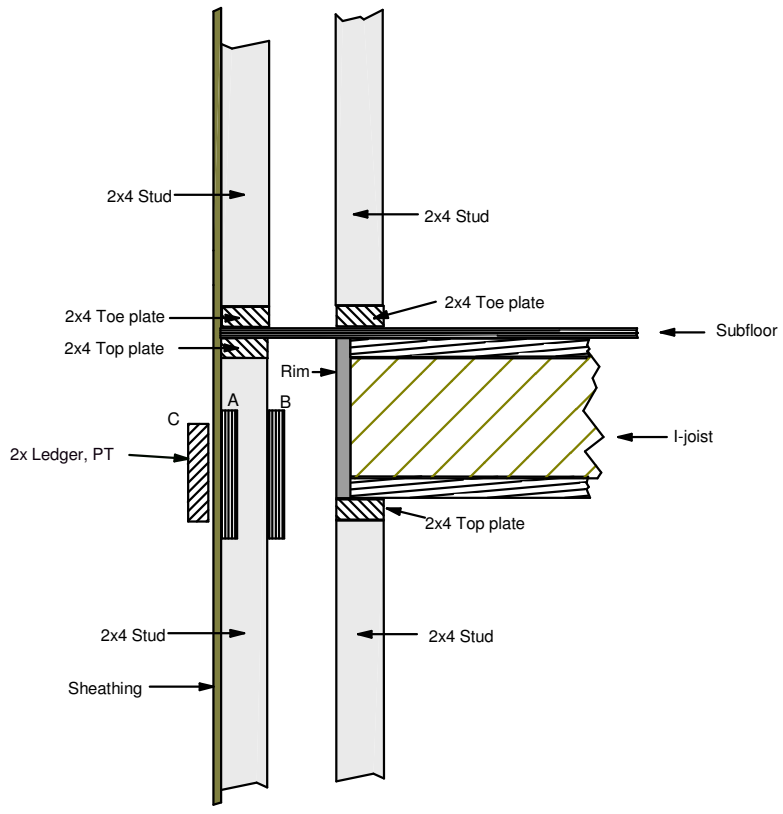
Deck Header Attachment to Double-Wall Framing (proposed)
