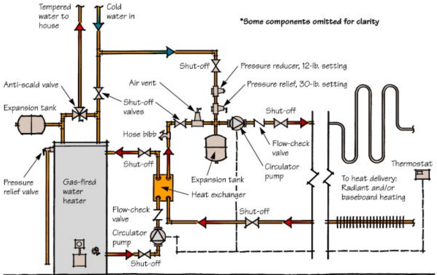
Figure 4. The author's favorite system uses an external heat exchanger to isolate the heating loop from the home's drinking water. The tank temperature is set high enough to meet the heating demand, while the domestic water is tempered for safety.
