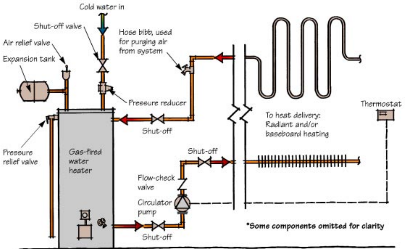
Figure 2. A dedicated setup is the simplest, least expensive way to use a water heater for space heating. The author always uses a unit with side taps for easy installation. The pump is installed at the bottom to avoid air lock.
