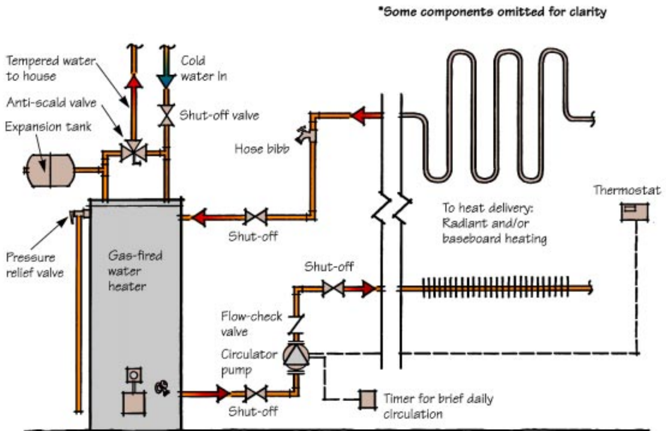
Figure 3. The dual-purpose setup provides both space heating and domestic water heating. The timer on the circulator shunts water through the heating loop at regular intervals to prevent the growth of bacteria that might take place if the water were stagnant.
