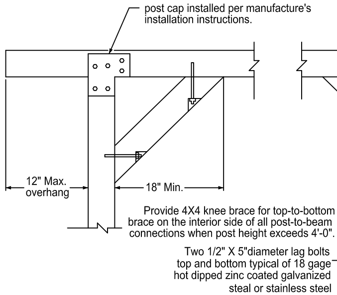
Figure 4 / Typical Deck Elevation Looking Parallel to Rear of Dwelling
