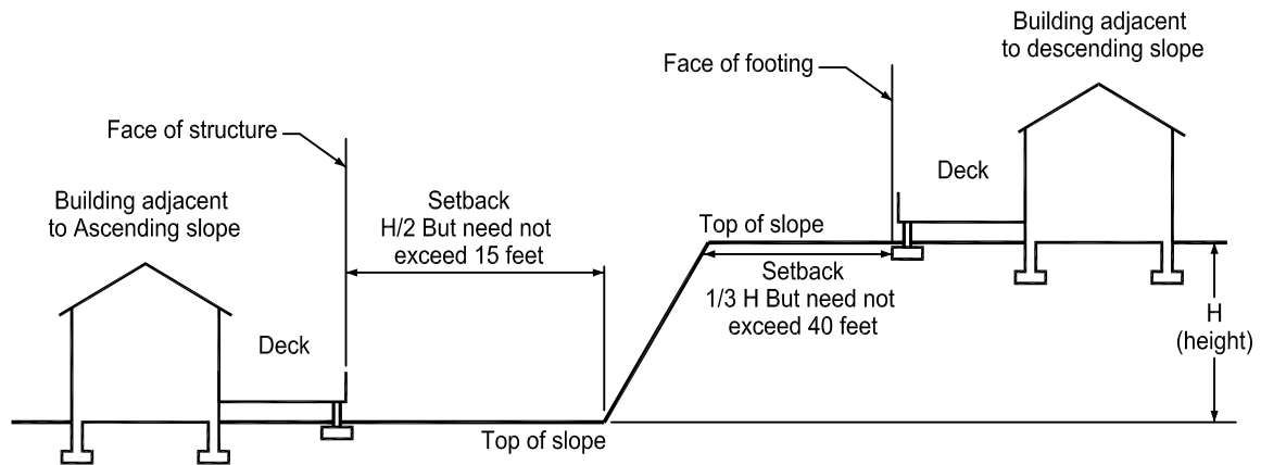
Figure 1 / Structures On or Adjacent to Slopes Foundation clearances from slopes
