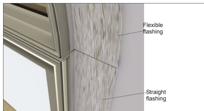
Figure 12 Use flexible flashing for radius head jambs.
