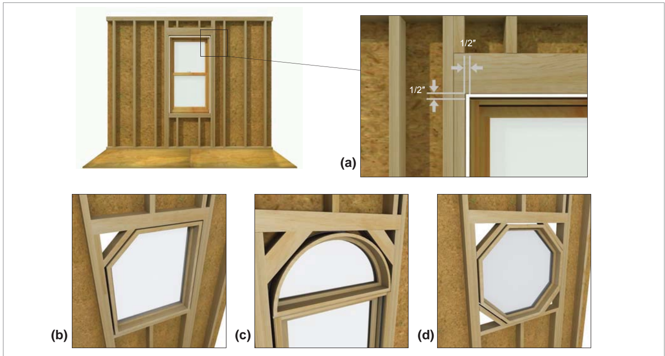
Figure 1 Typical rough and masonry openings.
