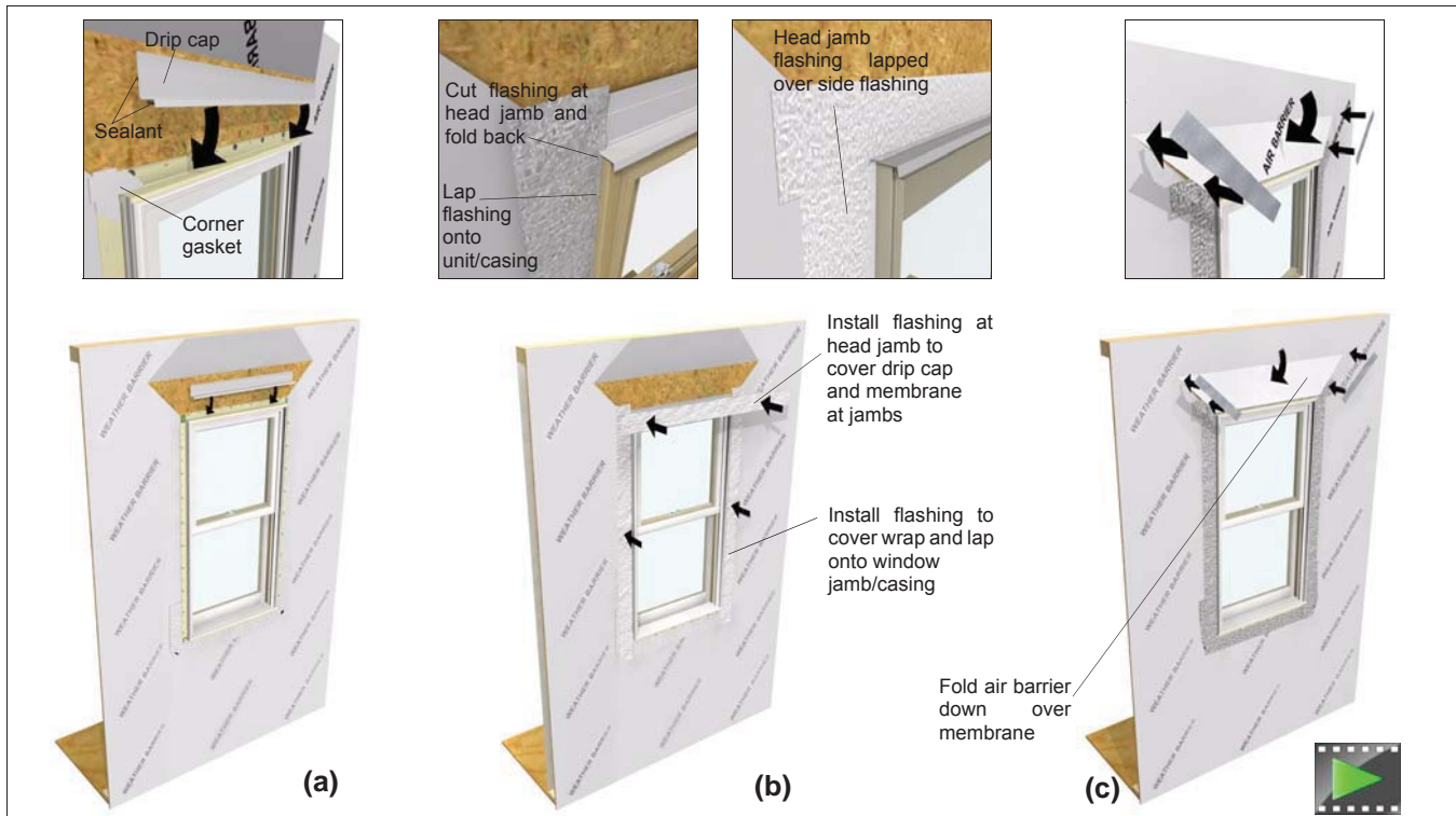
Figure 11 Sealing the Installation in air barrier applications. Click illustration to view video.
