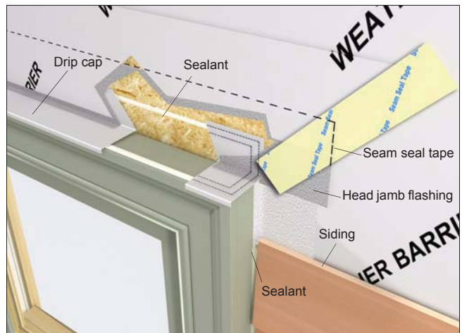
Figure 16 Apply perimeter sealant between window and exterior finish.
