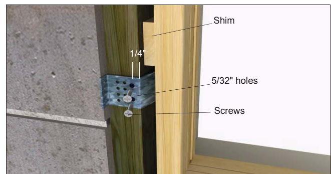
Figure 9 Attaching window with masonry clips or installation brackets.
