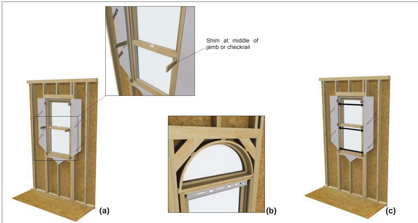
Figure 10 Shimming and squaring the window.
