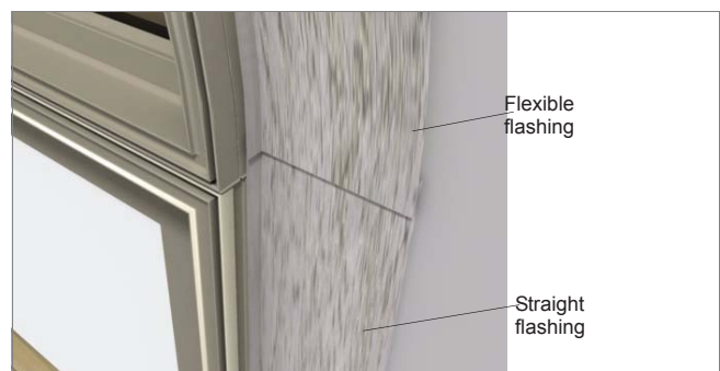
Figure 14 Use flexible flashing for radius head jambs.
