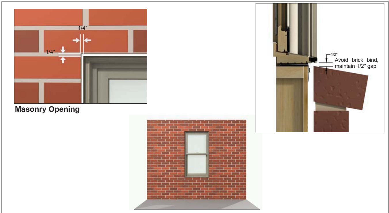
Figure 2 Typical rough and masonry openings.
