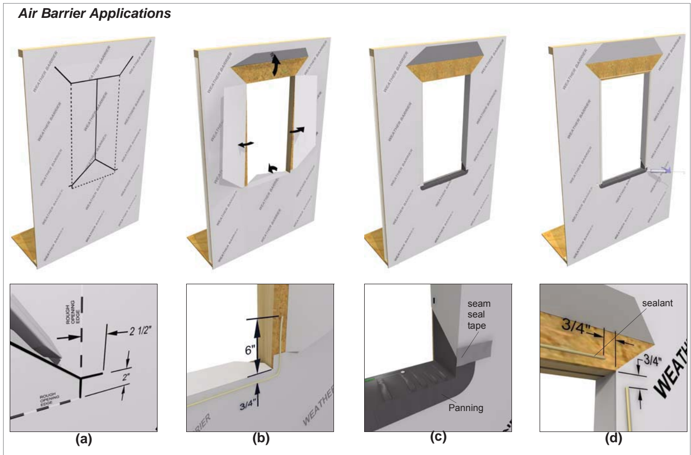
Figure 3 Rough Opening Preparation for construction methods using a continuous air barrier system and sill panning.
