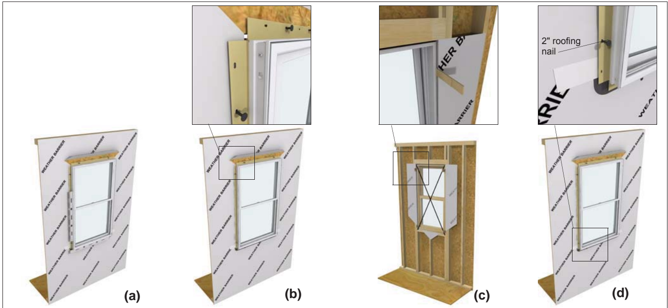
Figure 8 Positioning the window in the opening.
