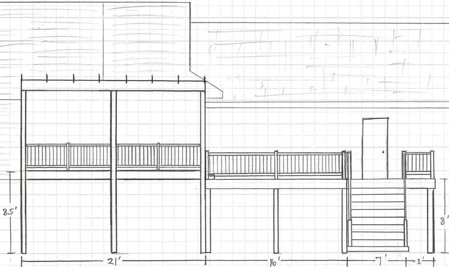
Front Elevation 3/16'' = 1 \text{ Ft}
