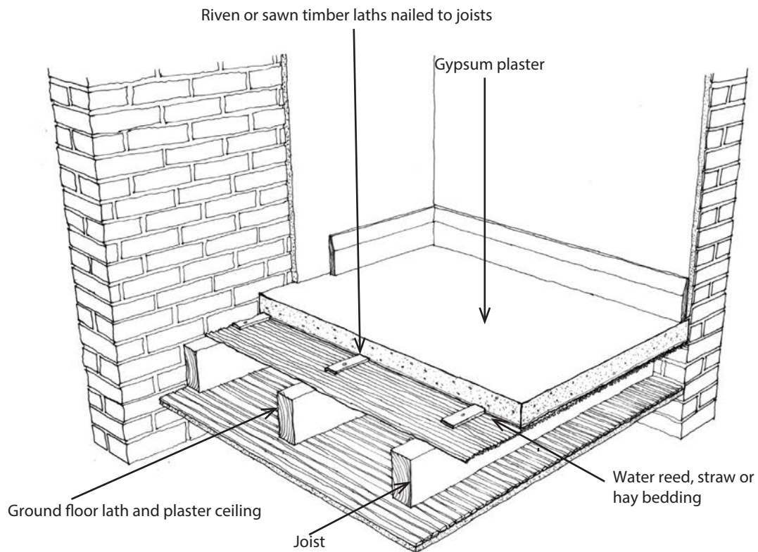
Figure 7: Cutaway of a typical gypsum plaster floor. Illustration: Ross Perkin
