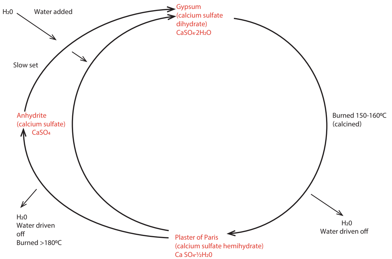
Figure 6: The gypsum cycle: heating of raw material and recrystallisation of hemihydrate and anhydrite back to gypsum. Illustration: SPAB
