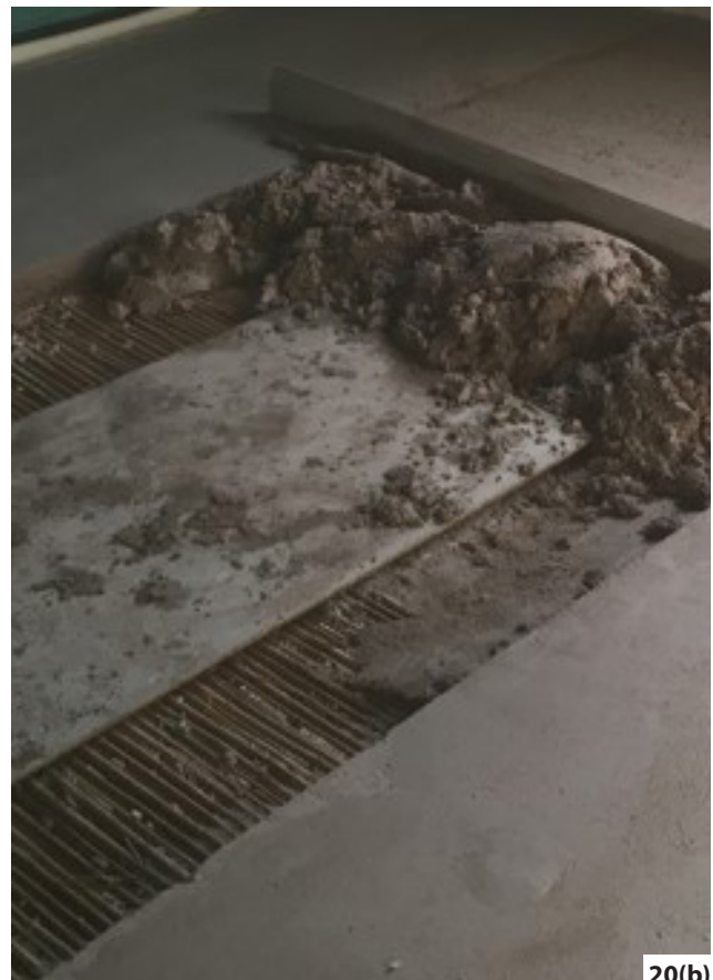
Figure 20: New gypsum plaster being laid between temporary timber battens (a) before the adjacent sections are infilled (b).
