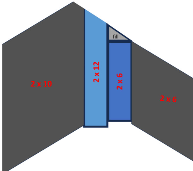
Proposed Sistered Ridge Board
